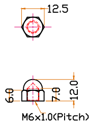
DOME NUT(M6x1.0mm Pitch)
