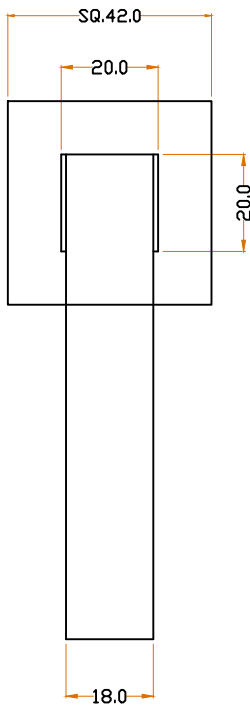
FRONT VIEW
