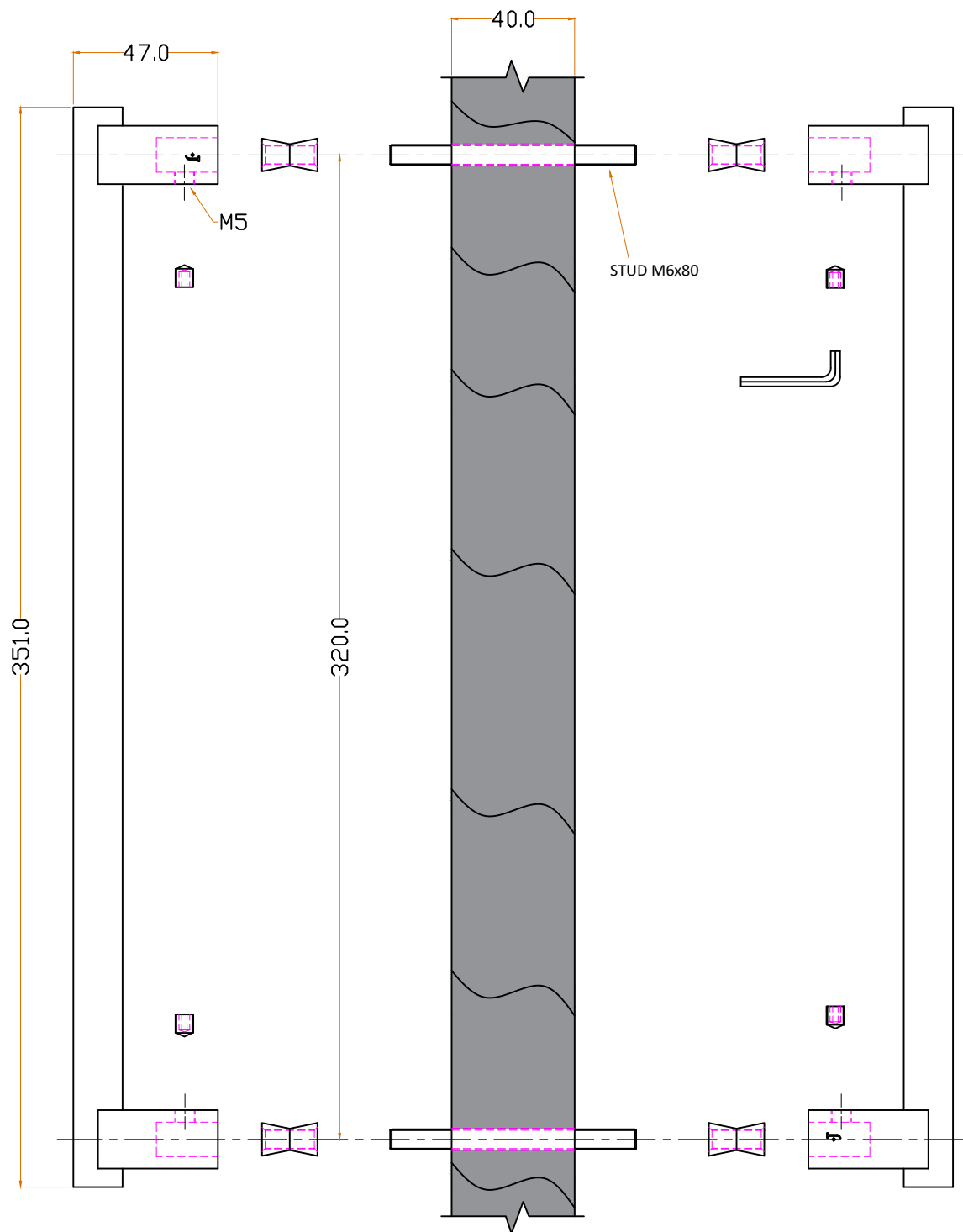
EXPLODED VIEW
